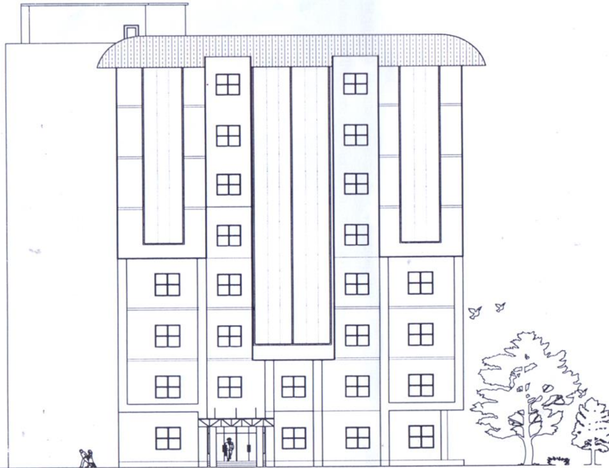
FRONT ELEVATION
